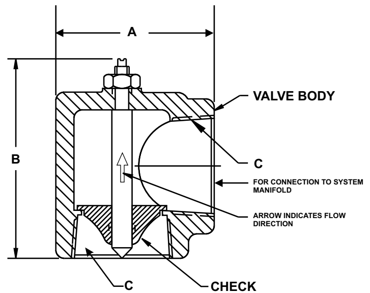
Figure 1. Manifold EI-Checks
