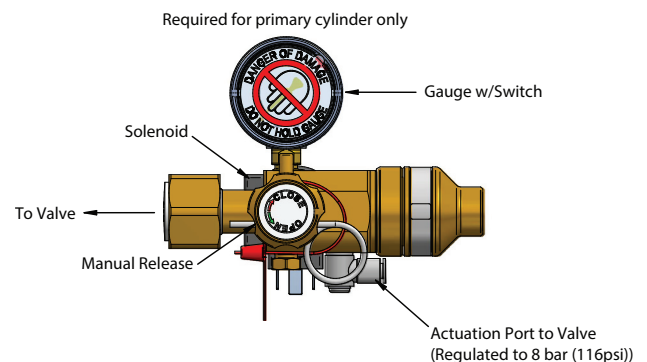
Figure 4. Release Unit
