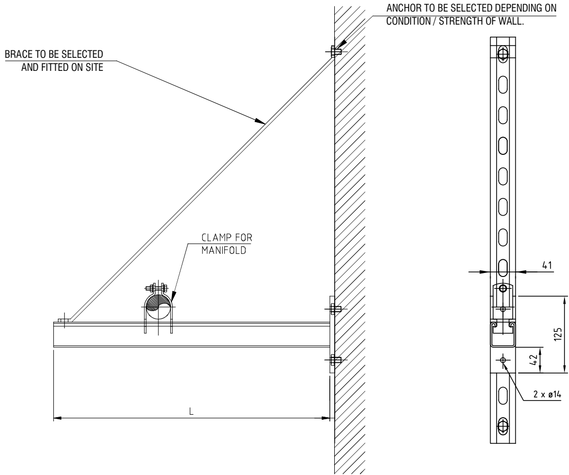
Figure 1. Manifold Installation
