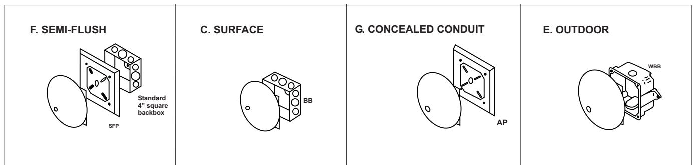
Figure 1. Mounting Details
