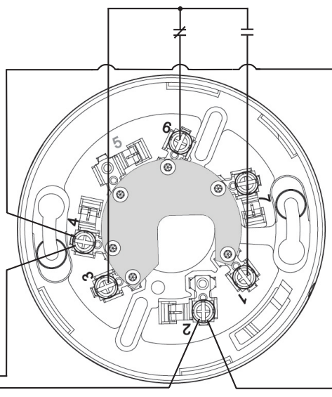
DS-SB Standard Base (Shown with Class B Wiring and Optional Remote LED)
