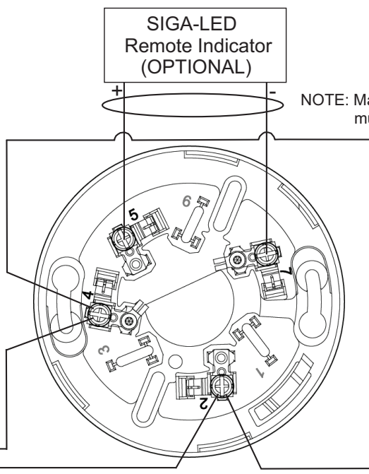
DS-SB Standard Base (Shown with Class B Wiring and Optional Remote LED)
